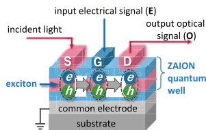
Fig. 1. Schematic diagram of an exciton transistor "EXOT".
